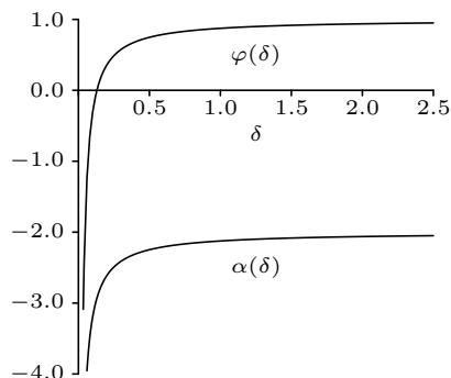
FIGURE 3. Plot of the coefficients \alpha(\delta) and \varphi(\delta) , defined in (3.58 d) on the range 0 < \delta < 2.5 .
