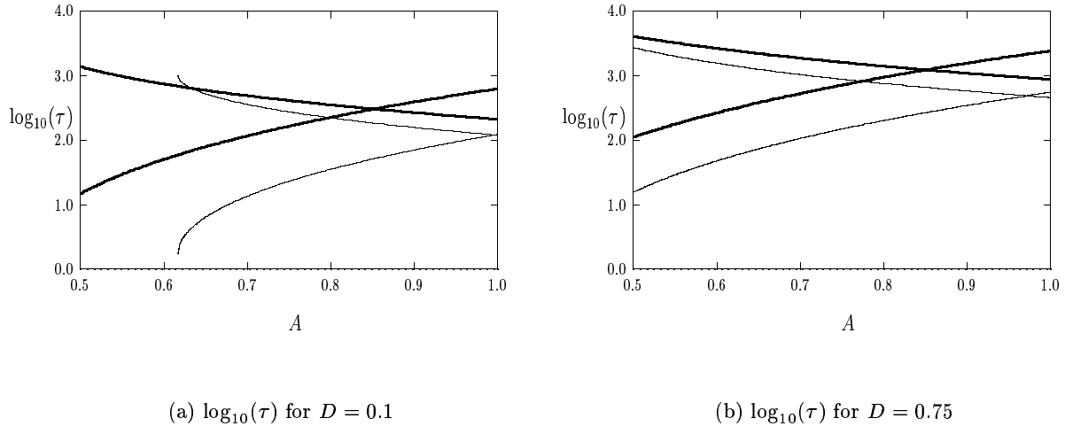
Figure 11: Plots of \log_{10}(\tau_H) (increasing curves) and \log_{10}(\tau_{TW}) (decreasing curves) as a function of A on the range \varepsilon^{1/2}\mathcal{A}_{1e} < A < 1 . The left figure and right figures are for D = 0.1 and D = 0.75 , respectively. The heavy solid curves are for \varepsilon = 0.005 and the solid curves are for \varepsilon = 0.01 .
