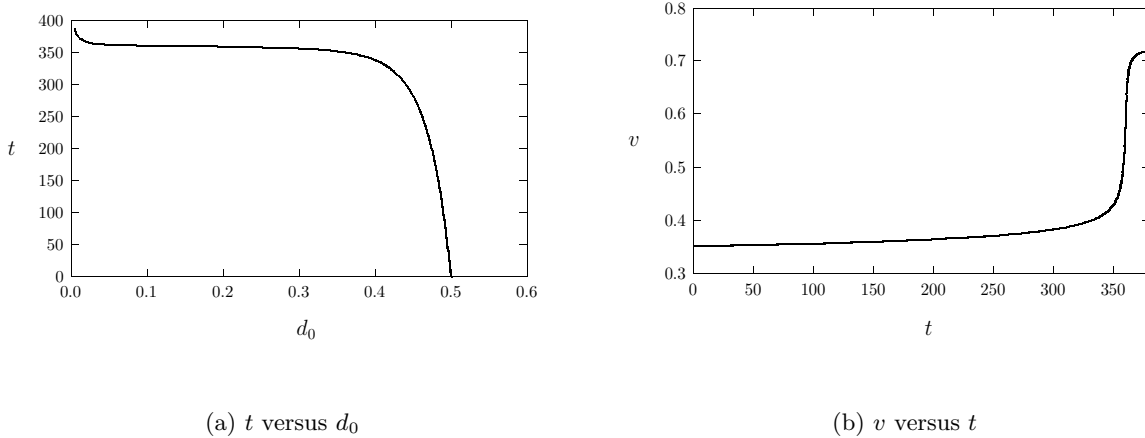
FIGURE 5. Numerical solution of (4.22) with \varepsilon = 0.11 for the flame-front tip in the unit disk. Left figure: the distance d_0(t) of the flame-front tip to the boundary. Right figure: the speed v(t) of the flame-front.
