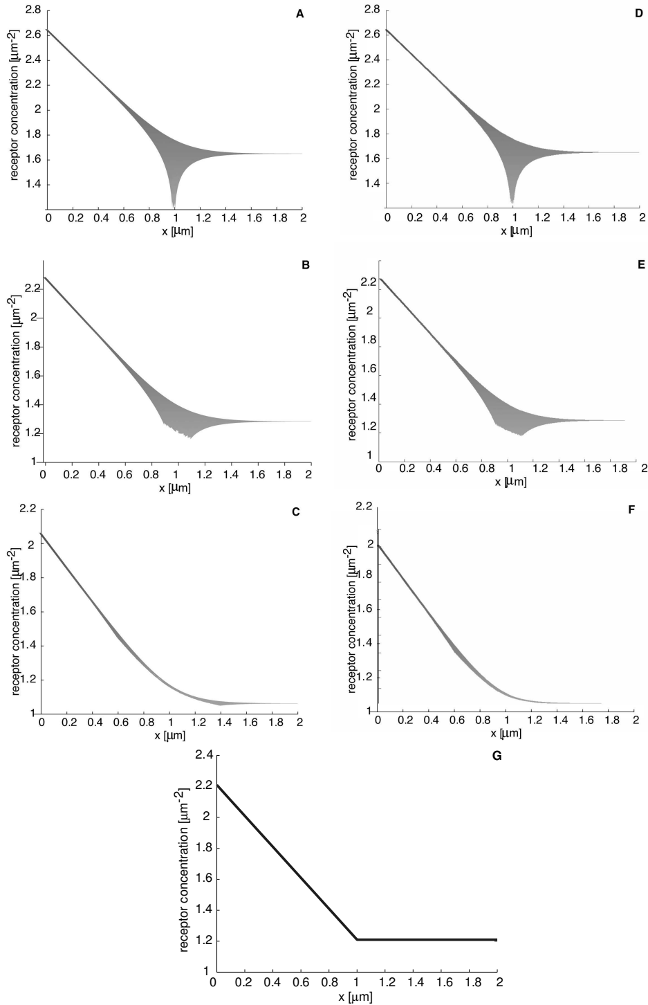
FIG. 4.3. Effect of spine radius \varepsilon on the solution U for a single spine on a short dendritic cable. (A-C) Plots of bulk dendritic receptor concentration U given by the outer solution (3.29) of the matched asymptotic expansion for parameter values as given in the text and \varepsilon = 0.01, 0.1 and 0.4 , respectively. The shaded region shows the range of values taken by the receptor concentration around the circumference of the cable as a function of distance x from the soma. (D-F) Corresponding plots of numerical solutions for U . (G) Plot of the one-dimensional solution [6].
