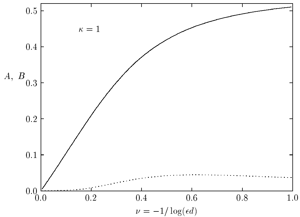
Figure 2: Plots of A and B versus \nu = -1/\log(\epsilon d) obtained from (2.16) when \kappa = 1 and d = e^{-1} . The solid line is A and the dotted line is B .
