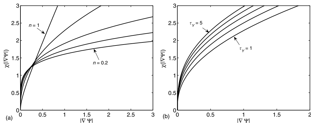
FIGURE 2. Examples of the function \chi(|\nabla\Psi|) for a Herschel–Bulkley fluid: (a) H = 1 , \tau_Y = 1 , \kappa = 1 , n = 1, 1/2, 1/3, 1/4, 1/5 ; (b) H = 1 , \tau_Y = 1, 2, 3, 4, 5 , \kappa = 1 , n = 1/2 .
