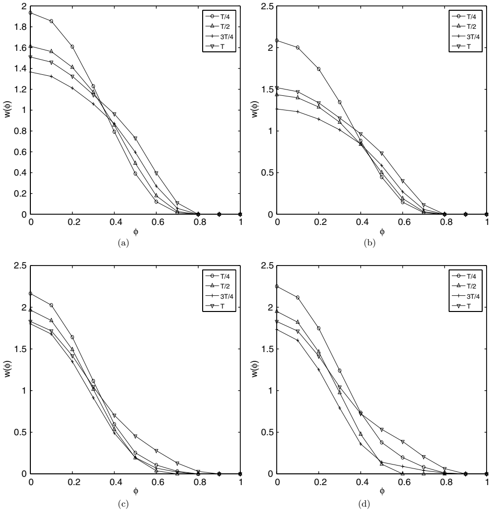
FIGURE 12. Velocity profile at \zeta = 1.5 : (a)–(b) Pseudo-steady model, \delta_p = 0.1, 0.2 , respectively. (c)–(d) Transient model, \delta_p = 0.1, 0.2 , respectively.
