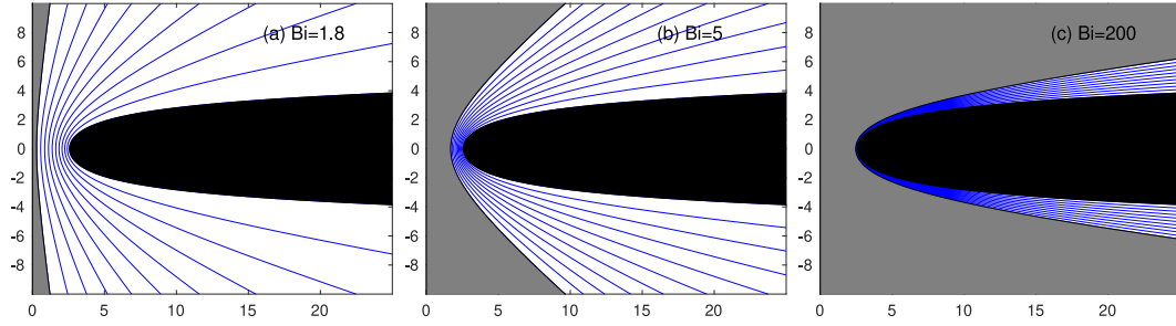
Fig. 9. Oldroyd's solution for flow of a Bingham fluid driven by a catenary moving past a plane wall for the three values of Bi indicated. Shown are contours of constant w , with the plug shaded grey and the catenary in black.
