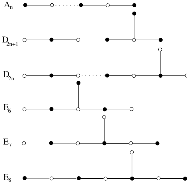
FIGURE 1. The set of binary roots of an ADE root system is the subset of the simple roots corresponding to the black nodes in the above Dynkin diagrams. The ADE Dynkin diagrams are dual to the configurations of exceptional curves in \widehat{S} . The map f : \widehat{S} \rightarrow Y contracts exactly the curves corresponding to binary roots.
