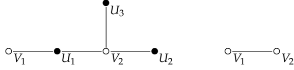
FIGURE 3. The intersection graphs of \widehat{\pi}^{-1}(0) and \pi^{-1}(0) respectively.
