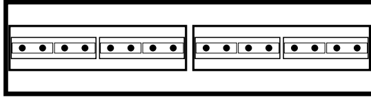
FIGURE 1. One dimensional hierarchical lattice
