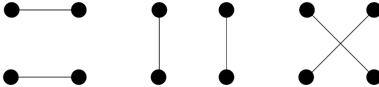
FIGURE 1. The three possible pairings for \int \prod_{i=1}^4 \varphi(x_i) d\mu .
