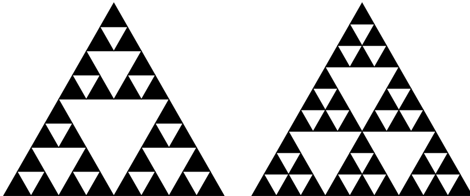
Figure 1: The first stages in the construction of SG(2) and SG(3)
