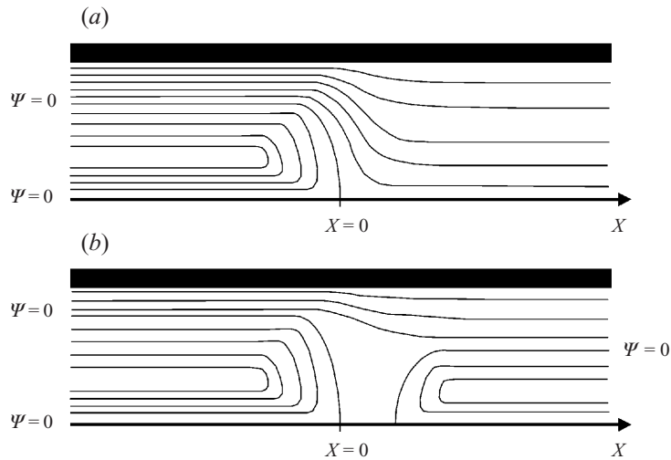
FIGURE 14. Schematic illustration of the two types of streamline behaviour: (a) no recirculation in fluid 2; (b) with recirculation in fluid 2.
