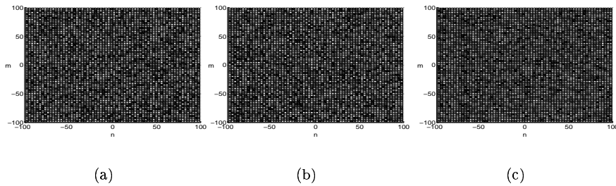
FIG. 6 The quantized frame coefficients q_{n,m} –obtained via the second-order scheme. Figure 6a shows the real part of the quantized coefficients; Figure 6b shows the imaginary parts of the quantized coefficients –black corresponds to -10 and white corresponds to 10 in these figures. Figure 6c shows the absolute value of the quantized coefficients; in this figure black corresponds to 0 and white corresponds to 10\sqrt{2} .
