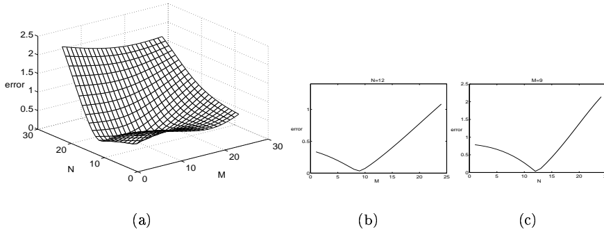
FIG. 8 The value \langle \tilde{F}_{T,\Omega,A,2} - I_{N,M}, G_{tot} \rangle versus N and M for T = 1.2 and \Omega = 0.9 ; the minimum is obtained at N = 12 and M = 9 , which means that the algorithm predicts T = 1.2 and \Omega = 0.9 , i.e. the correct values of T and \Omega . Figure 8b shows \langle \tilde{F}_{T,\Omega,A,2} - I_{12,M}, G_{tot} \rangle vs. M ; Figure 8c shows \langle \tilde{F}_{T,\Omega,A,2} - I_{N,9}, G_{tot} \rangle vs. N .
