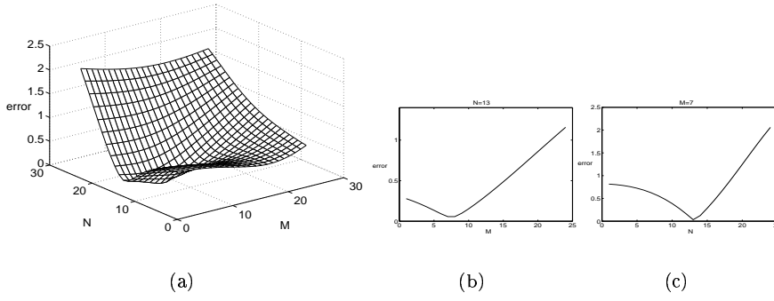
FIG. 4 The value \langle \tilde{F}_{T,\Omega,A} - I_{N,M}, G_{tot} \rangle versus N and M for T = 1.2 and \Omega = 0.9 ; the minimum is obtained at N = 13 and M = 7 , which means that the algorithm predicts T = 1.3 and \Omega = 0.7 . Figure 4b shows \langle \tilde{F}_{T,\Omega,A} - I_{13,M}, G_{tot} \rangle vs. M ; Figure 4c shows \langle \tilde{F}_{T,\Omega,A} - I_{N,7}, G_{tot} \rangle vs. N .
