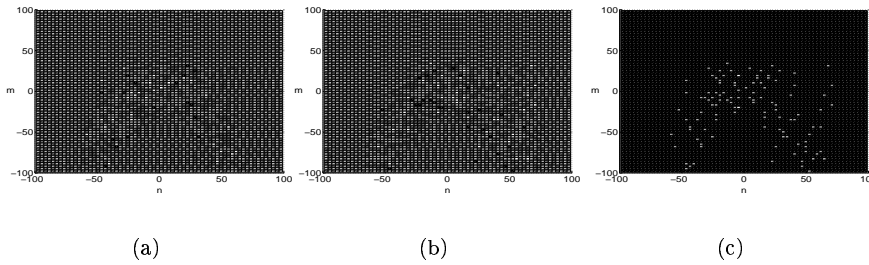
FIG. 2 The quantized frame coefficients \langle f, \varphi_{n,m} \rangle for the frame (\varphi, 0.1, 0.1) . Figure 2a shows the real part of the quantized coefficients; Figure 2b shows the imaginary parts of the quantized coefficients; Figure 2c shows the absolute value of the quantized coefficients. In Figures 2a and 2b black and white correspond to -3 and 3 respectively. In Figure 2c black corresponds to \sqrt{2} and white corresponds 3\sqrt{2} .
