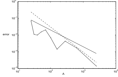
FIG. 3 The ‘approximation error’ |\langle F - \tilde{F}_A, G_{tot} \rangle| vs. the frame bound A . Both axes are logarithmic. The solid line seen in the figure is the graph \{(A, 2A^{-1}) : 25 < A < 1258\} ; the dashed line is the graph \{(A, 30A^{-3/2}) : 25 < A < 1258\} .
