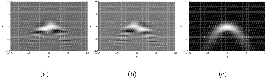
FIG. 1 The continuous windowed Fourier transform F of f , i.e. F(\tau, \xi) = \langle f, \varphi_{\tau, \xi} \rangle . Figure 1a shows the real part of F –black and white correspond to -0.49 and 0.75 , respectively ; Figure 1b shows the imaginary part of F –black and white correspond to -0.57 and 0.69 , respectively. Figure 1c shows the absolute value of F . In this graph, black corresponds to 0 and white corresponds to 0.86 .
