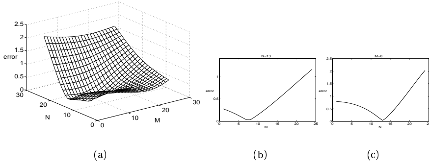
FIG. 5 The value \langle \tilde{F}_{T,\Omega,A} - I_{N,M}, G_{tot} \rangle versus N and M for T = 1.17 and \Omega = 0.93 ; the minimum is obtained at N = 13 and M = 8 , which means that the algorithm predicts T = 1.3 and \Omega = 0.8 . Figure 5b shows \langle \tilde{F}_{T,\Omega,A} - I_{13,M}, G_{tot} \rangle vs. M ; Figure 5c shows \langle \tilde{F}_{T,\Omega,A} - I_{N,8}, G_{tot} \rangle vs. N .
