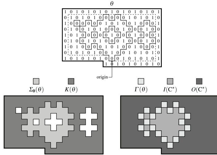
FIGURE 2. A configuration \theta \in E_{C^*} . On the left, the associated sets \Sigma_0(\theta) and K(\theta) . On the right, the sets I(C^*) and O(C^*) for \Gamma(\theta) = C^* .
