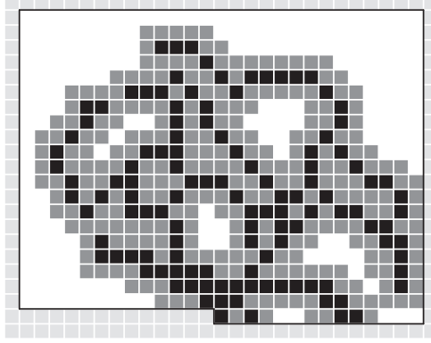
FIGURE 1. A \star -connected \Theta (in black), the set \Delta = \partial^* \Theta \cap \Lambda (in dark grey) and \Lambda^c (in light grey) for \Lambda = S_{y,z} .
