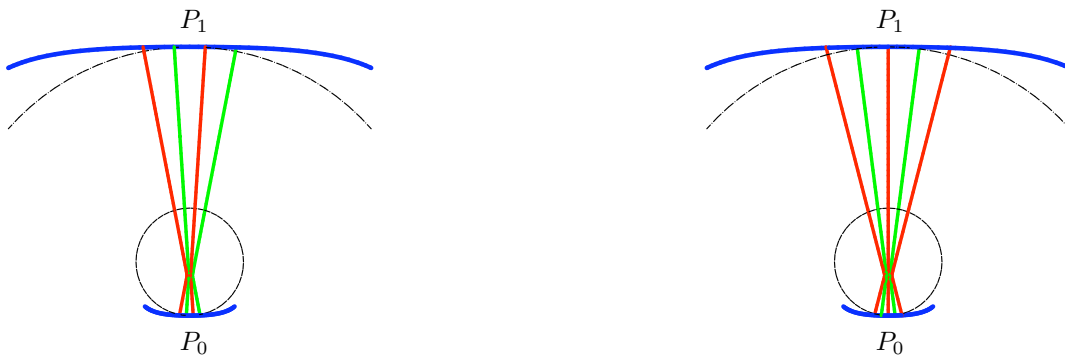
Figure 2: Equilibrium configurations as in Figure 1 with \ell = 1 , R_0 = \frac{1}{5} , R_1 = \frac{9}{10} and \varepsilon = \frac{1}{25} .
