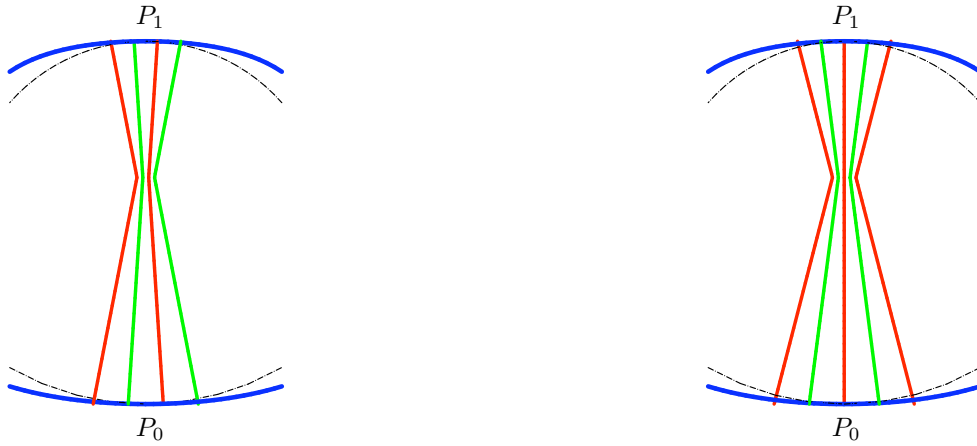
Figure 1: Equilibrium configurations of 4 and 5 interfaces with \ell = 1 , R_0 = \frac{3}{4} , R_1 = \frac{1}{2} and \varepsilon = \frac{1}{25} . The dotted lines indicate the osculating circles of the boundary at points P_0 and P_1 respectively.
