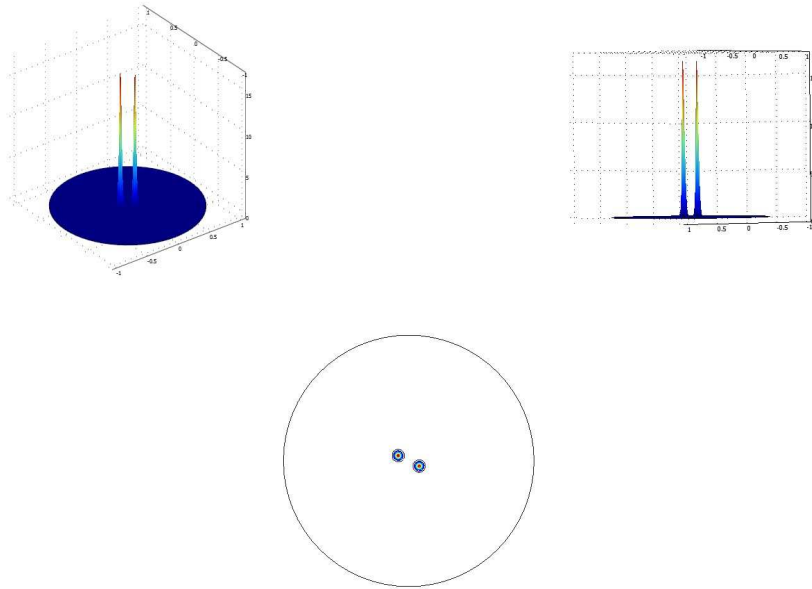
Figure 2. Clustered spiky steady state of (1.2) for \varepsilon^2 = 0.001 , D = 0.01 , \mu(|y|) = 1 + 5|y|^2 . Shown is a 2-spike cluster consisting of 2 spikes on a regular polygon. The activator A is displayed in two three-dimensional surface plots from different perspectives in the top two graphs and its projection to the domain plane is shown in the bottom graph.
