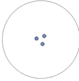
Figure 1. Clustered spiky steady state of (1.2) for \varepsilon^2 = 0.001 , D = 0.01 , \mu(|y|) = 1 + 5|y|^2 . Shown is a 3-spike cluster consisting of 3 spikes on a regular polygon. The activator A is displayed in two three-dimensional surface plots from different perspectives in the top two graphs and its projection to the domain plane is shown in the bottom graph.
