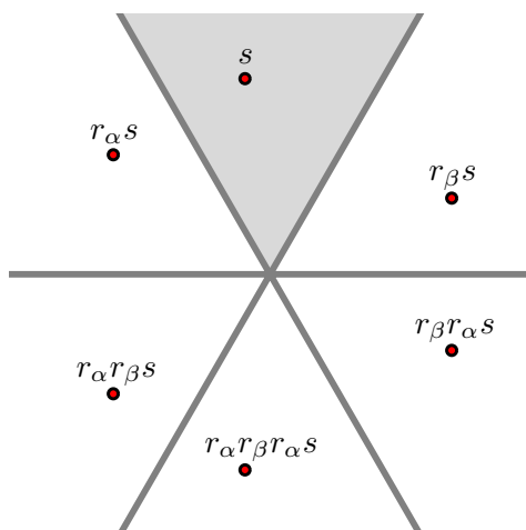
Figure 4. The Weyl group action for SL_3
