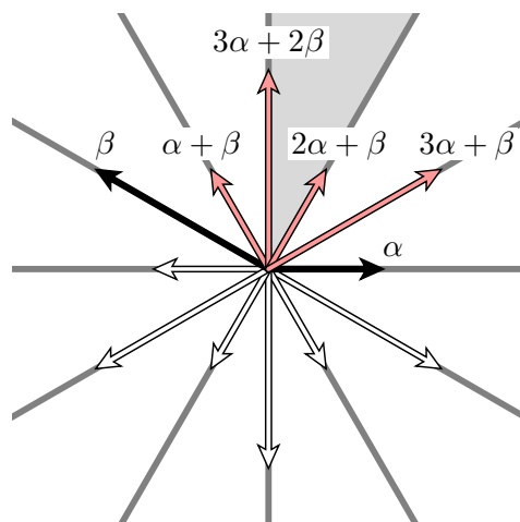
Figure 10. The root system G_2
