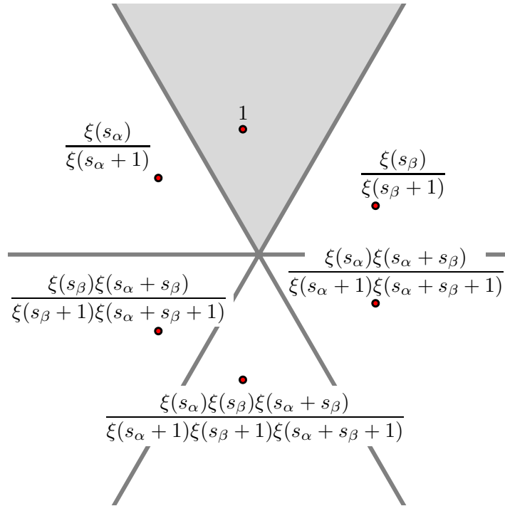
Figure 5. Coefficients for the constant term of E_s
