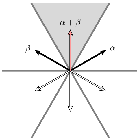
Figure 3. The root system for SL_3
