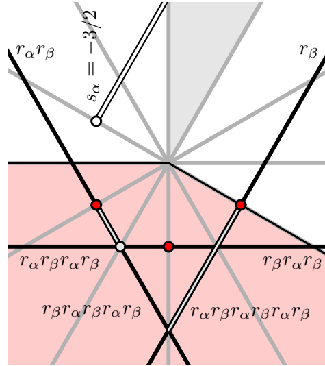
Figure 12. Constant term for the residue along s_\beta = 1
