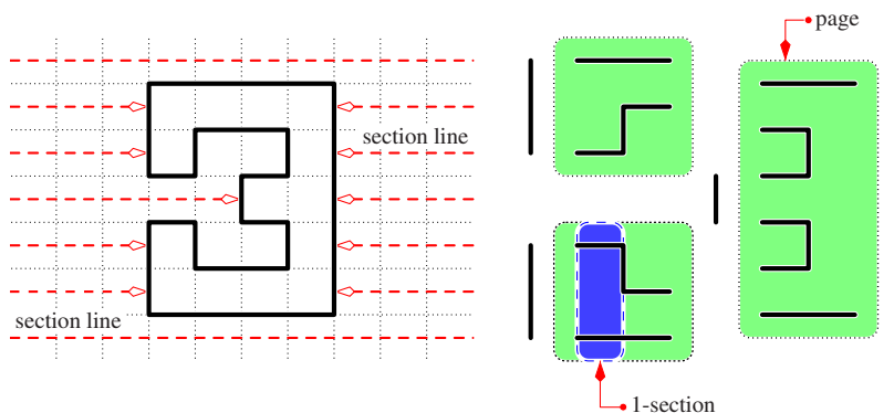
Fig. 2. Section lines (the heavy dashed lines in the left-hand figure) split the polygon into pages (as shown on the right-hand figure). Each column in a page is a section . This polygon is split into 3 pages, each containing 2 sections; a 1-section is highlighted. Ten vertical bonds lie between pages and 4 vertical bonds lie within the pages.
