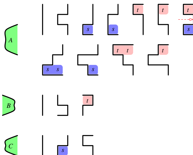
Fig. 15. The “frills” of the building blocks in Fig. 14.
