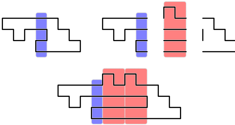
Fig. 8. To construct a polygon with 2M + 1 k -sections and 6k - 4 + 2M vertical bonds, start with a polygon with a single k -section and 6k - 4 vertical bonds as shown (top left). Cut it on the right of the k -section. Insert M copies of the pair of k -sections and recombine the polygon. This gives a polygon with 2M + 1 k -sections and 6k - 4 + 2M vertical bonds.
