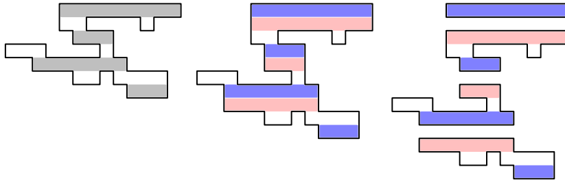
Fig. 10. Decomposing 2-4-2 polygons into building blocks. Highlight each row with 2 vertical bonds. Then “duplicate” each of these rows excepting the bottommost. By cutting along each of these duplicated rows each 2-4-2 polygon is decomposed into a rectangle (of unit height) and a sequence of building blocks.
