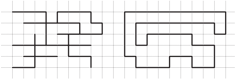
Fig. 1. A square lattice bond animal (left) and a self-avoiding polygon (right).
