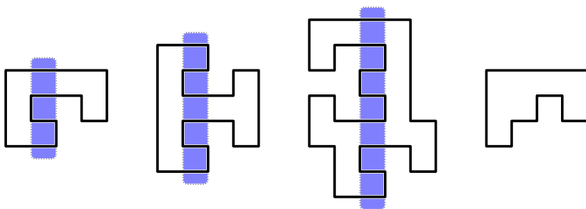
Fig. 9. Four section-minimal 2-4-2 polygons. The first three polygons contain a 2-section, a 3-section, and a 4-section, respectively. The rightmost polygon contains only 1-sections.
