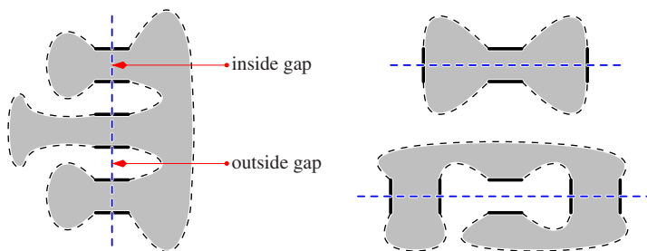
Fig. 4. Vertical and horizontal lines drawn through a k -section show the minimum number of vertical bonds required in their construction.
