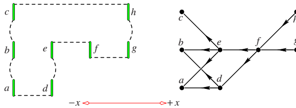
Fig. 13. The vertical bonds of a 2-4-2 polygon building block. The x -ordinate of these bonds are denoted a, b, \dots, h as shown. The Hasse diagram showing the constraints on the values a, b, \dots, h is given on the right; an arrow from v_i to v_j implies that v_i > v_j .
