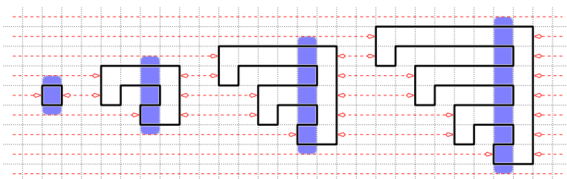
Fig. 5. Section-minimal polygons with 6k - 4 vertical bonds and a single k -section may be constructed by concatenating such “hook” configurations.
