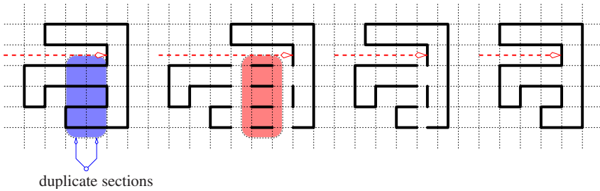
Fig. 3. The process of section deletion. The two indicated sections are identical. Slice either side of the duplicate and separate the polygon into three pieces. The middle piece, being the duplicate, is removed and the remainder of the polygon is recombined. Reversing the steps leads to section duplication. Also indicated is a section line which separates the duplicate sections from the rest of the columns in which they lie.
