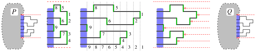
Fig. 6. Given an sm-polygon P we can create a new sm-polygon Q that is identical to P except for the region lying to the right of its rightmost k -section; that region is altered to maximise the number of sections lying to the right of the k -section. We do this by stretching that portion P that lies to the right of the k -section so that no two vertical bonds lie in the same vertical line. The polygon is then made section-minimal again by deleting duplicate sections.
