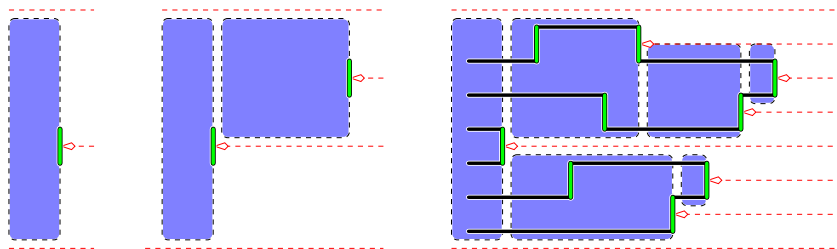
Fig. 7. The pages in the stretched polygon before removing duplicate sections. By “scanning” from left to right we see that each page corresponds one vertical bond that blocks a section line.
