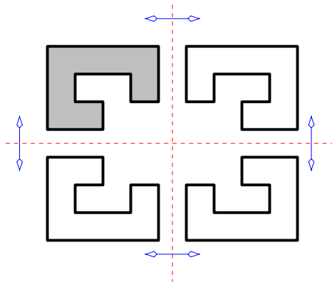
Fig. 12. The set of building blocks has a 4-fold symmetry as shown. It suffices to find all the building blocks in one orientation and then obtain the others by reflections.
