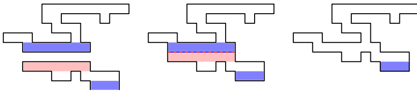
Fig. 11. Constructing a 2-4-2 polygon from a (shorter) 2-4-2 polygon and a 2-4-2 building block. Note that when the building block and the polygon are squashed together, the total vertical perimeter is reduced by 2, and the total horizontal perimeter is reduced by twice the width of the joining row.
