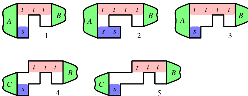
Fig. 14. The section-minimal building blocks of 2-4-2 polygons. The “frills”, denoted A, B and C are given in Fig. 15.
