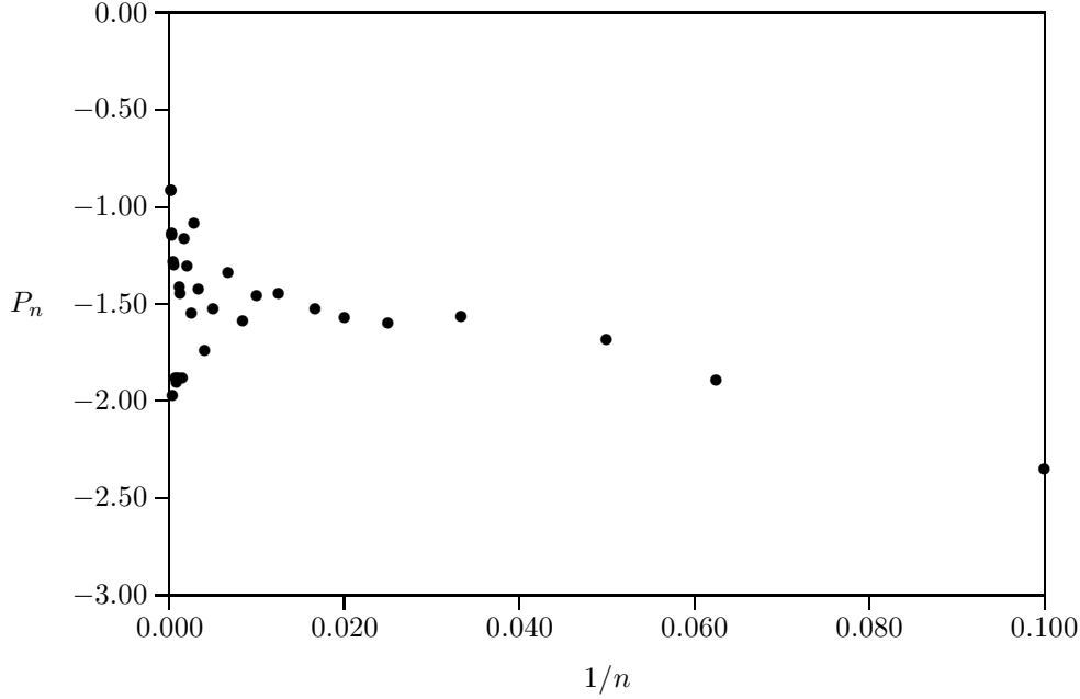
Figure 5. Scatterplot of P_n = n \left( \log \left( \frac{\langle a_+ \rangle}{\langle a_- \rangle} \right) - \log \mu^2 \right) against 1/n . Error bars have been left away for clarity. \mu^2 was set equal to its least squares value in equation (30). The data points accumulate around -1.5 ; this is consistent with \alpha = 1/2 .
