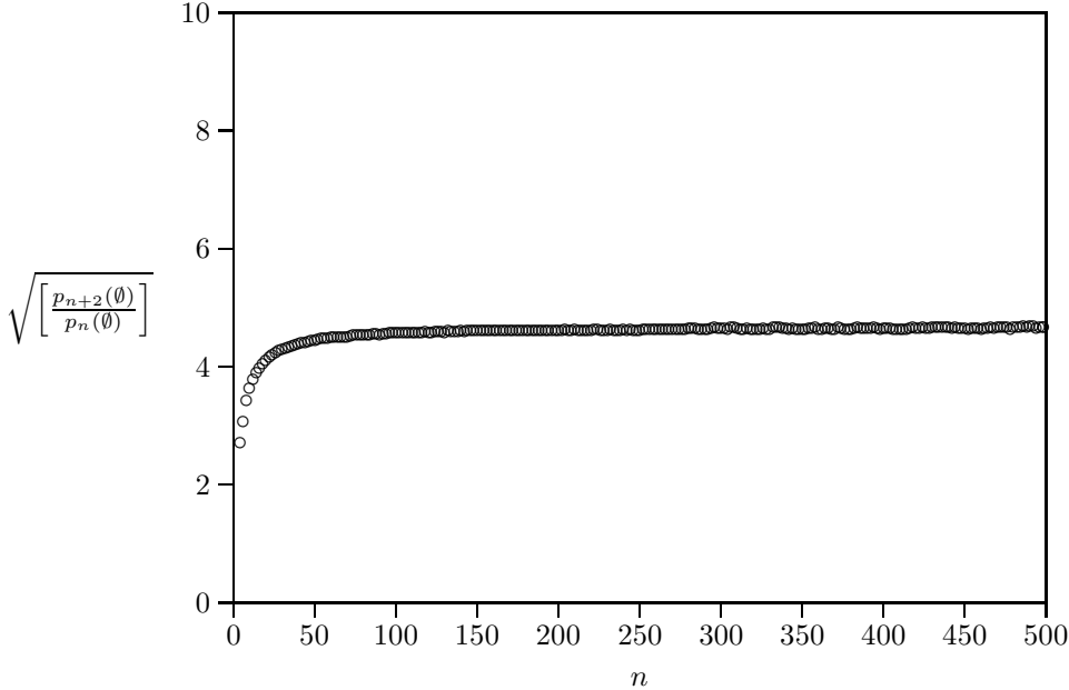
Figure 8. The ratio [p_{n+2}(\emptyset)/p_n(\emptyset)]^{1/2} against n for unknotted polygons. Note that the data appears to be monotonically increasing to a limiting value.
