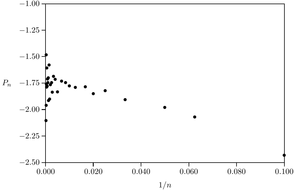
Figure 7. Scatterplot of P_n = n \left( \frac{\langle a_+ \rangle}{\langle a_+ \rangle} - \log \mu^2 \right) against 1/n . Error bars have been removed for clarity. \mu^2 was set equal to its least squares value in equation (39). The data points accumulate around -1.77 ; this is consistent with \alpha \approx 0.23 .
