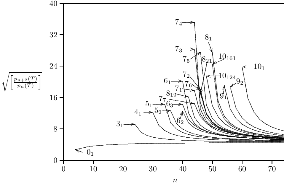
Figure 12. The ratio [p_{n+2}(T)/p_n(T)]^{1/2} against n for knotted polygons with crossing number up to ten. crossing knot types. Relative entropy at small values of n is large for 7_4 , 8_1 and 7_3 , amongst these knot types.
