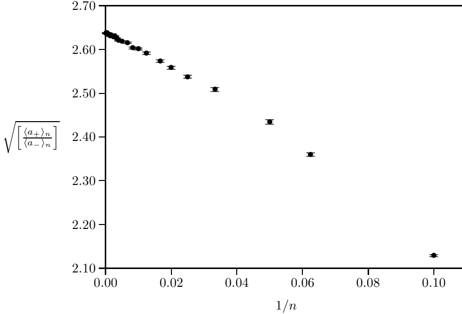
Figure 4. The ratio [\langle a_+ \rangle_n / \langle a_- \rangle_n]^{1/2} plotted against 1/n in the square lattice. Extrapolation of the data to infinite n is done by a regression with the model 2d-1 to estimate \mu .
