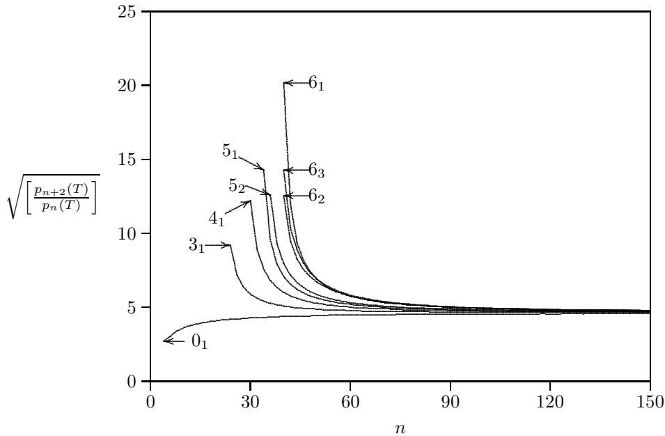
Figure 11. The ratio [p_{n+2}(T)/p_n(T)]^{1/2} against n for polygons of six crossing knot types. The most relative entropy is found in 6_1 and the least in the square knot and 6_2 , for small values of n . Observe that the square knot and 6_2 has virtually the same change in relative entropy with increasing n .
