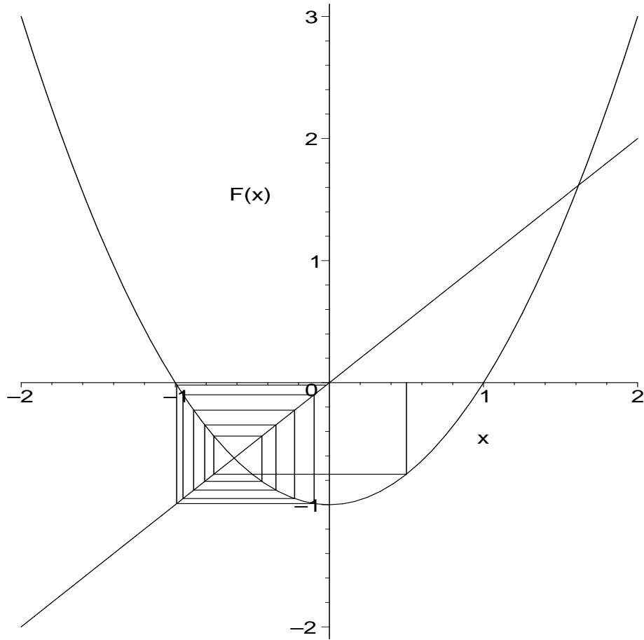
Iterates of x^2 - 1
